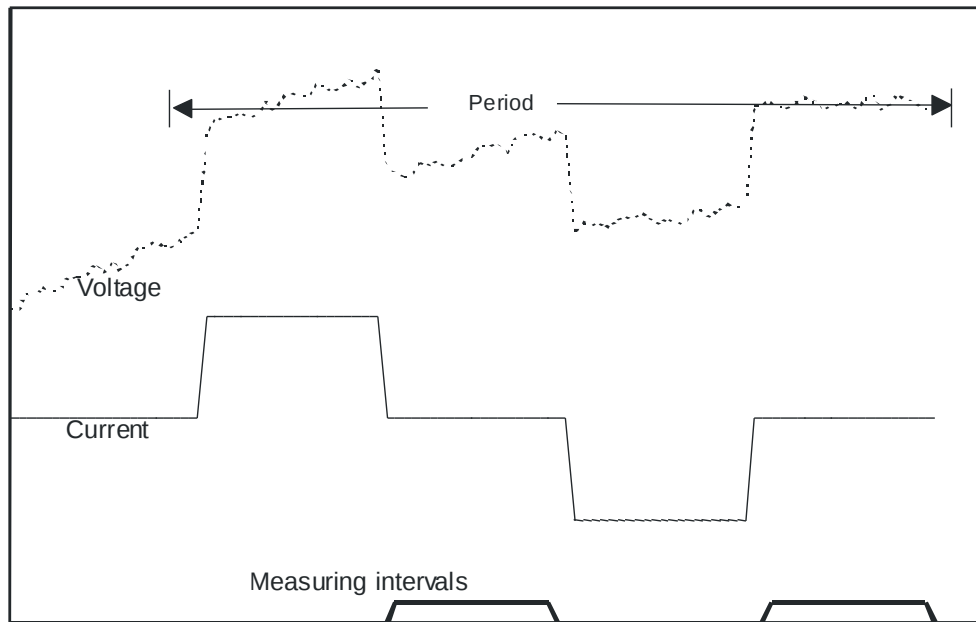
Figure 105 IP measuring cycle timing definitions
