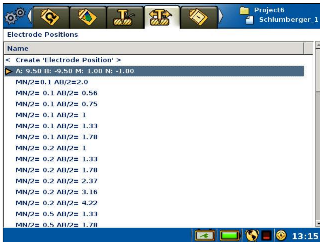
Figure 72 Result of Create Electrode Position
