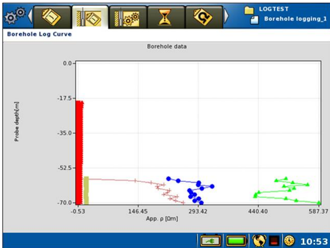
Figure 87 Borehole Log Curve View
