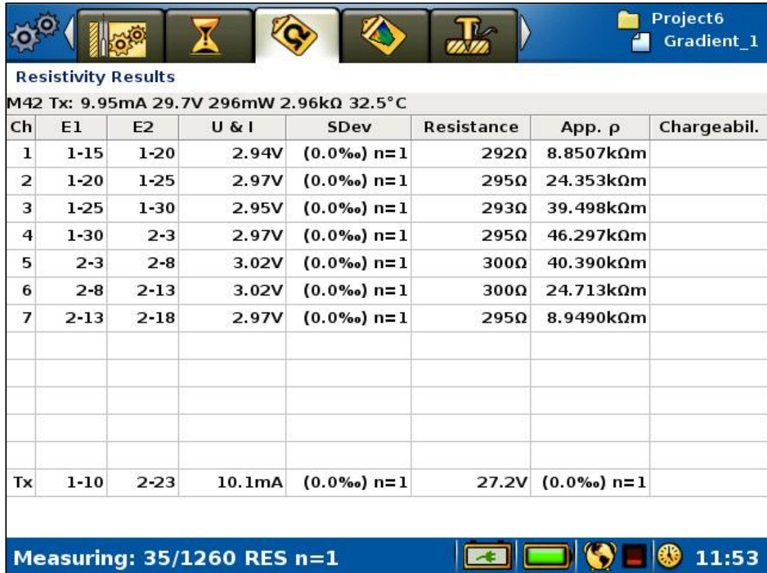
Figure 61 Resistivity results view
