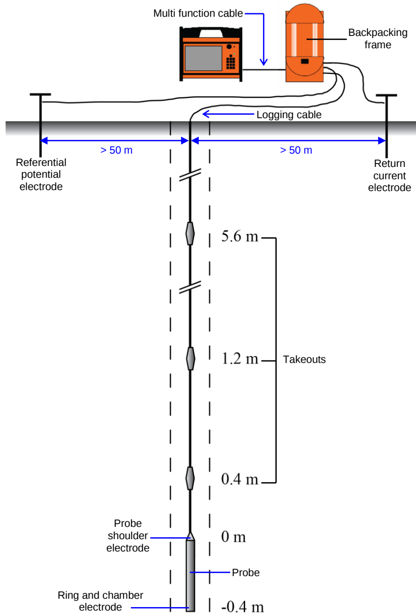
Figure 79 Overview of cabling and layout of the electrodes
