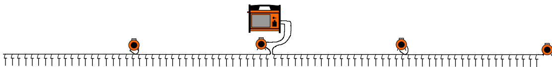
Figure 52 Cable arrangement at the second measurement station in a roll-along survey
