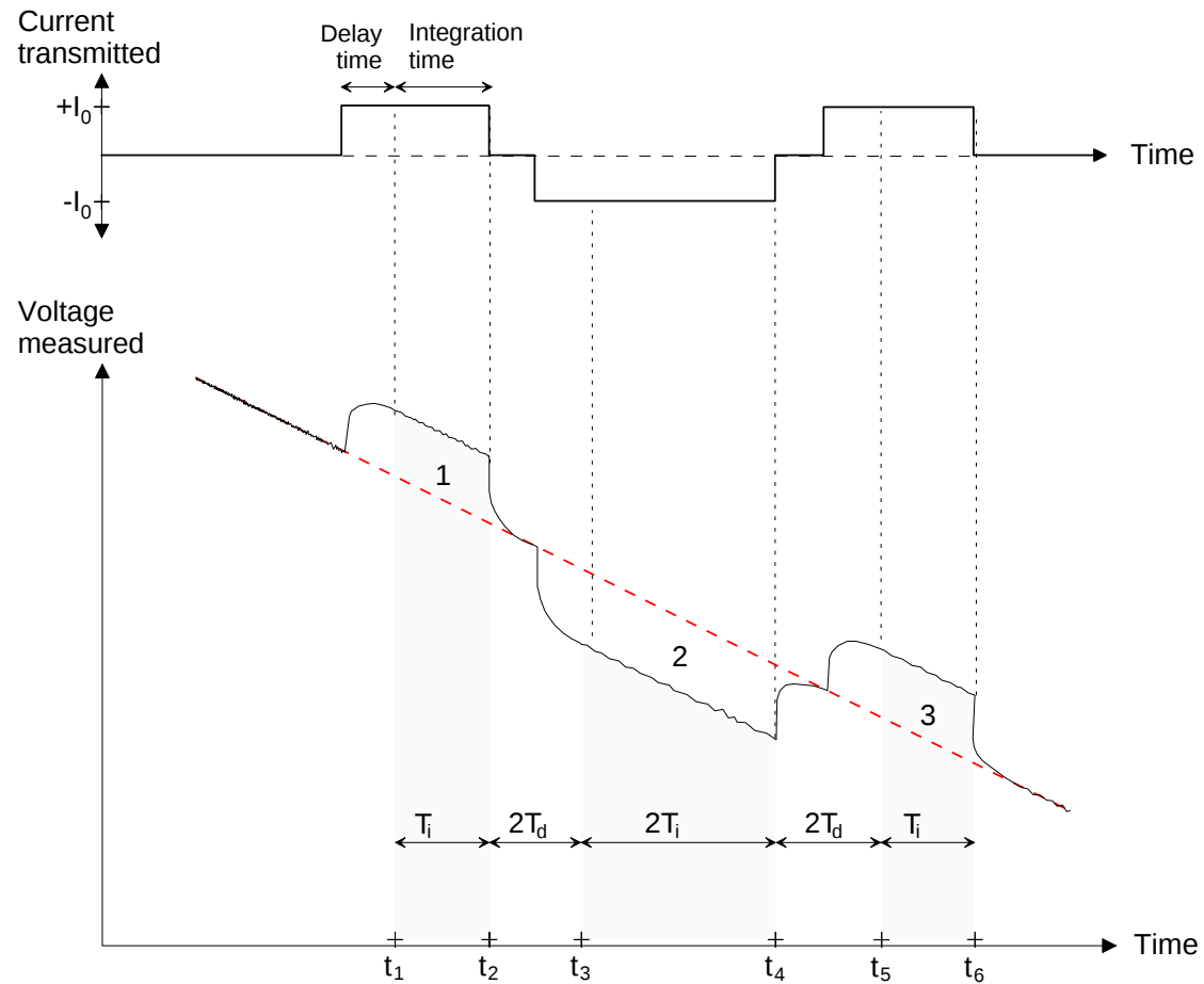
Figure 104 Resistivity measuring cycle timing definitions (after Krill 1977)
