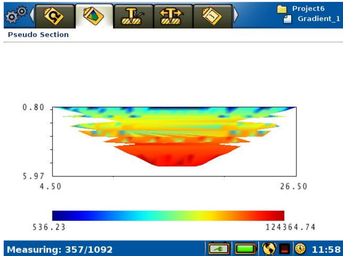
Figure 62 Pseudo section view
