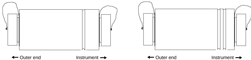
Figure 51 Cable joints with connection direction for, a) 4 x 21 take-out cable set, b) 4 x 16 take-out cable set
