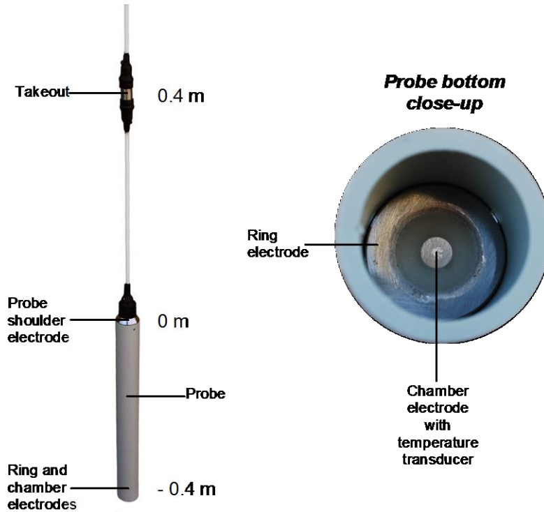
Figure 78 Logging probe with close-up of probe bottom
