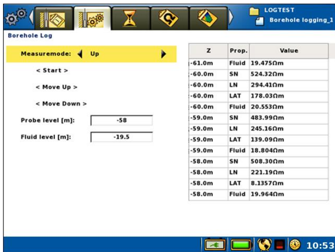
Figure 86 Borehole Log View – Table filled with measured values
