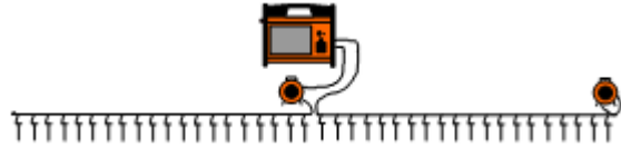
Figure 53 Cable arrangement at the last measurement station
